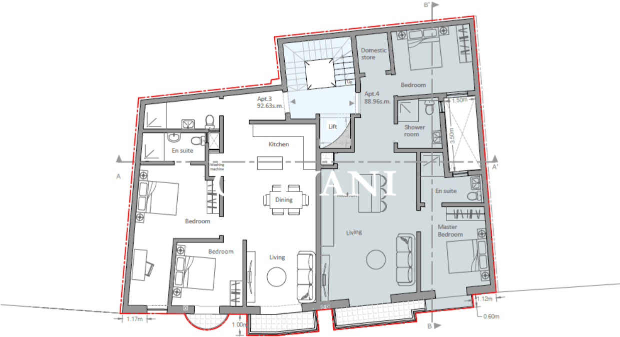
Proposed Second Floor 1:100
