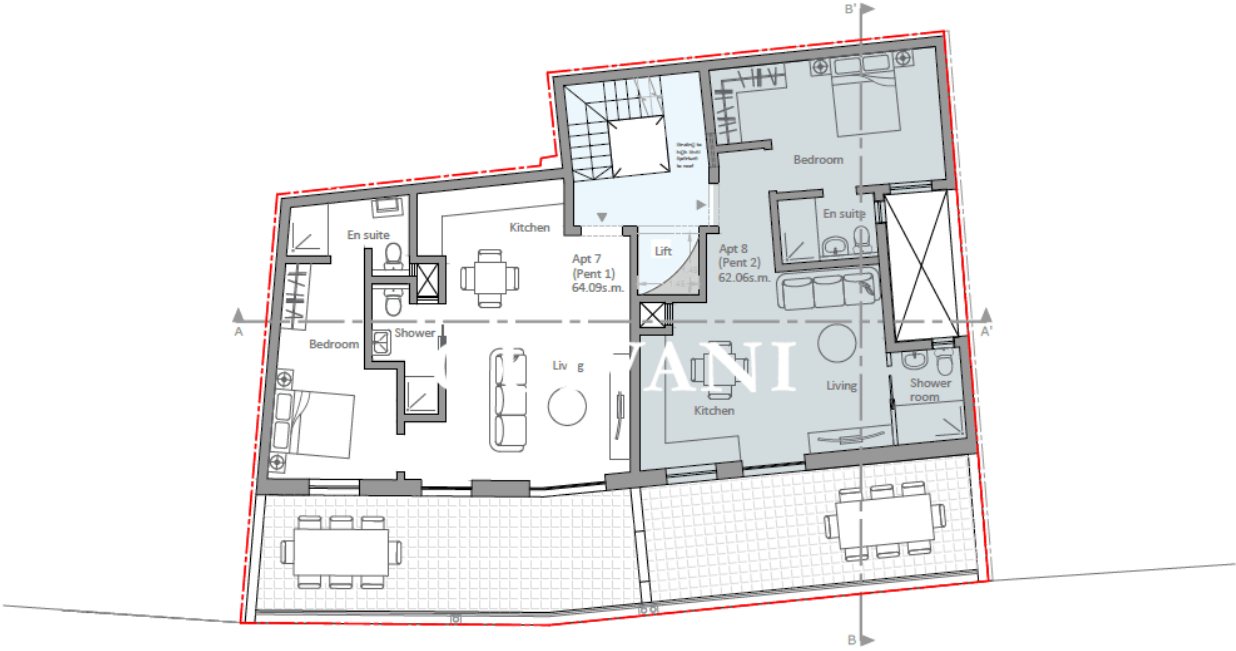
Proposed Fourth Floor (receded) 1:100
