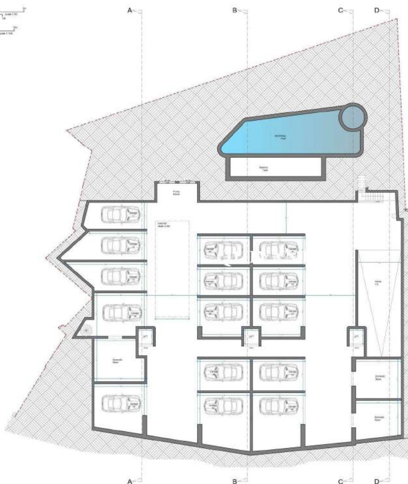
Lower Basement Floor Plan
