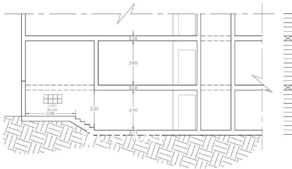
Proposed Section DD
