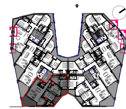
BLOCK PLAN
